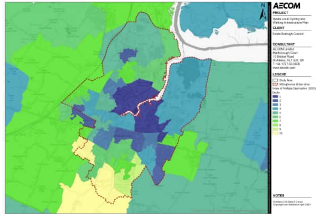
Figure 2-19 IMD- Sittingbourne
