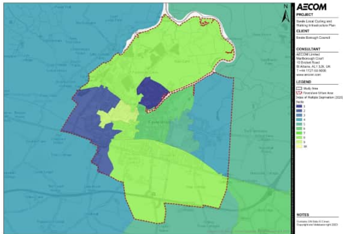
Figure 2-18 IMD- Faversham
